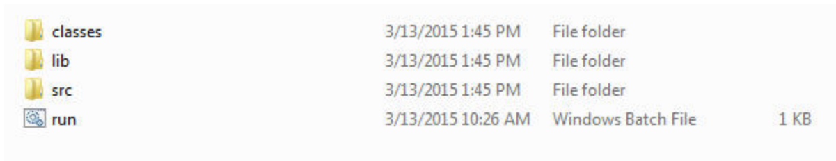
Figure 1-3 JavaQSR Files
