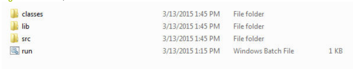
Figure 1-4 JavaPAT Files
